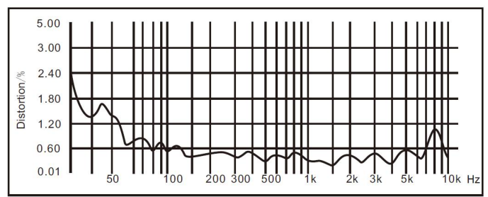
Distortion Characteristics (THD < 3% 1W, 1m, 100Hz-10kHz)
