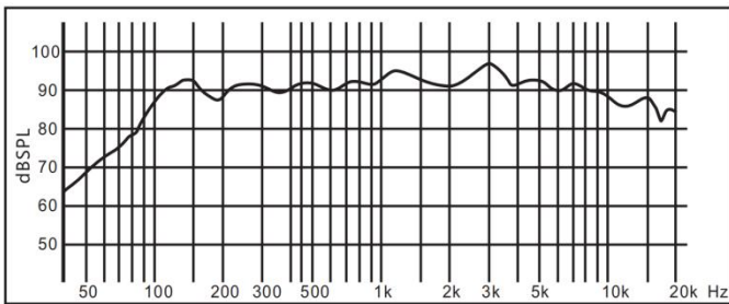
Frequency Response Characteristics (dB SPL, 1W, 1m)
